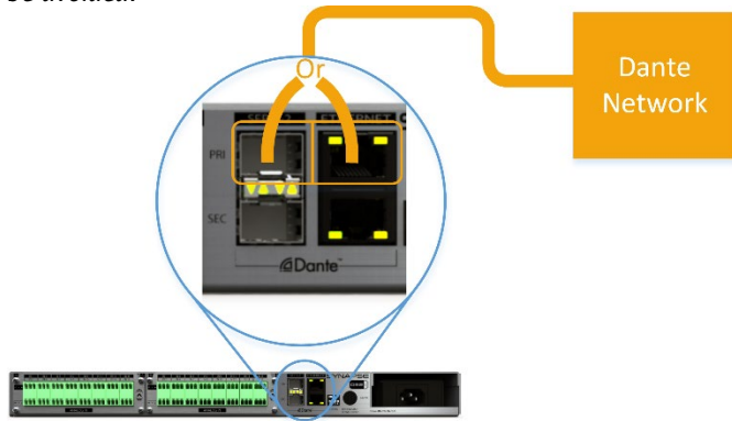
Figure 8 - "Standalone" connection in "Redundant" mode
