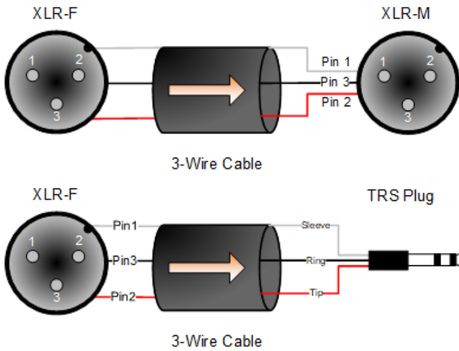
Figure 4 – Balanced Wiring Guide
