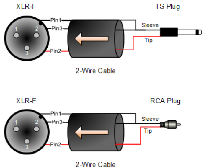
Figure 3 – Balanced Wiring Guide
