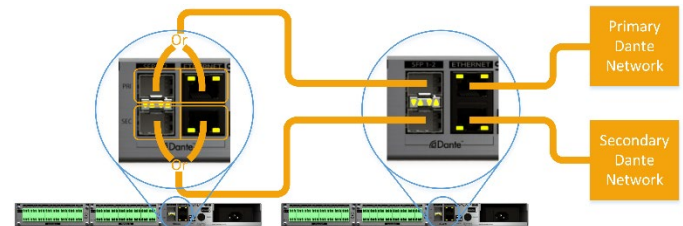
Figure 7 - "Redundant" mode with daisy chaining
