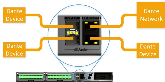
Figure 9 - "Standalone" connection in "Switched" mode
