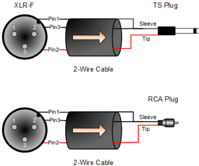
Figure 5 – Unbalanced Wiring Guide
