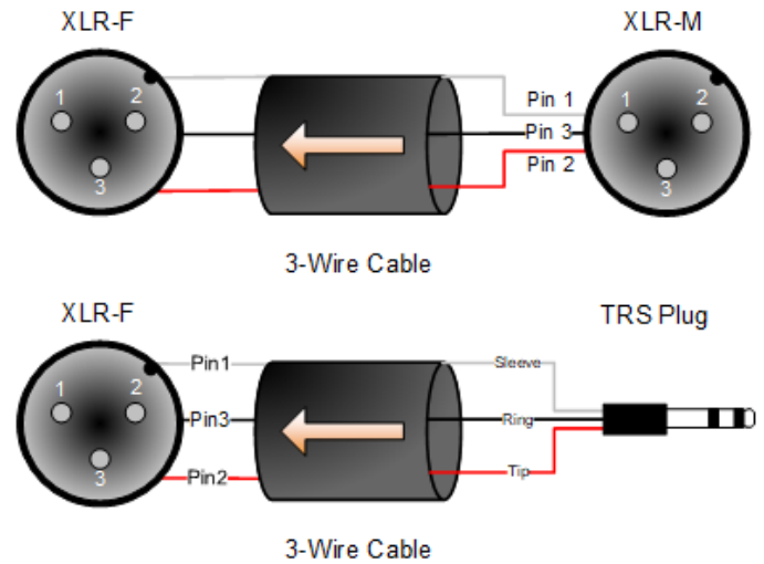
Figure 2 – Balanced Wiring Guide
