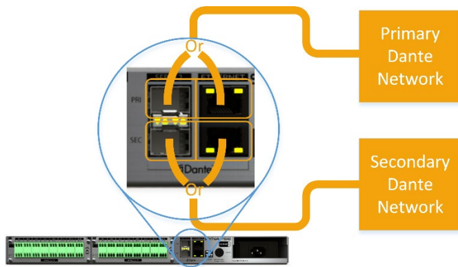
Figure 6 –"Redundant" mode, no daisy chain
